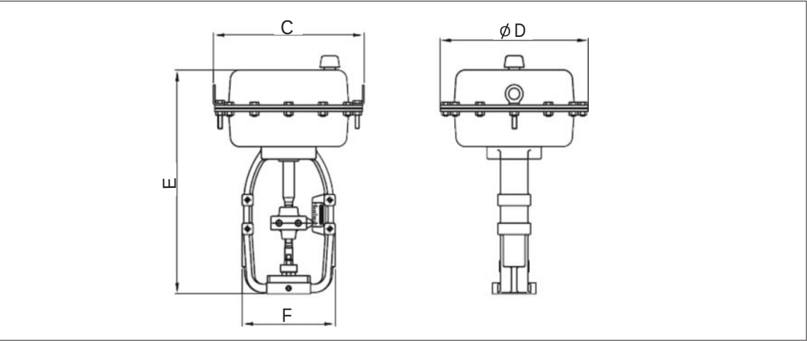
弹簧薄膜型执行机构尺寸 Sping and Diaphragm Actuator Dimension
